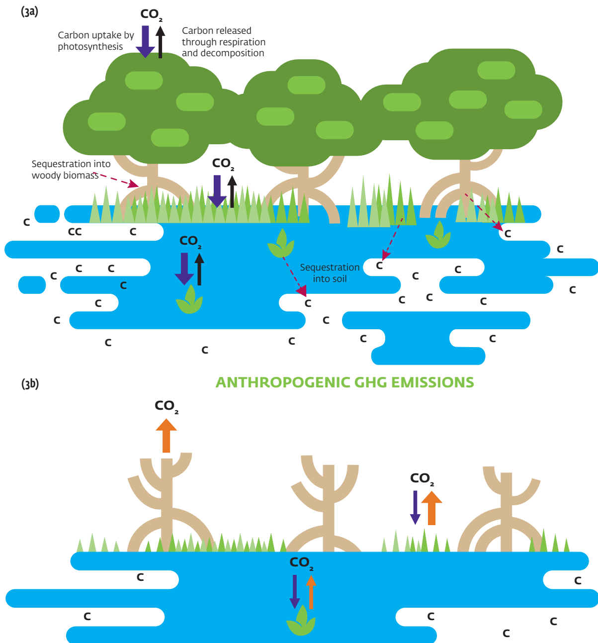
FIGURE 3: UPTAKE, STORAGE, AND RELEASE OF CO 2 IN COASTAL WETLANDS
